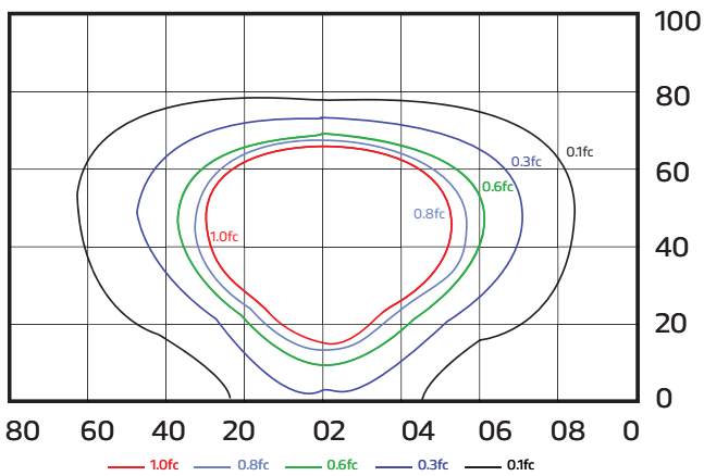
HYPER 25W TYPE III [ MOUNTING HETGHT 20FT ]
